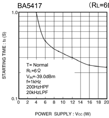
Fig.38 Starting time vs. Supply Voltage
