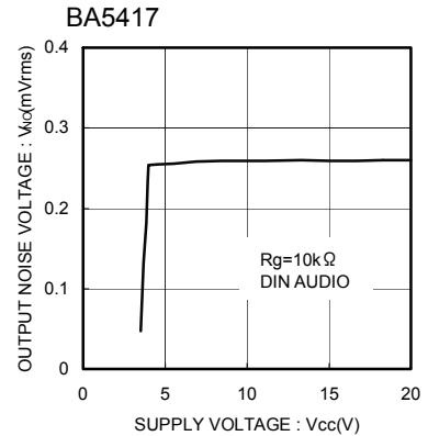
Fig.22 Output noise voltage vs Supply voltage
