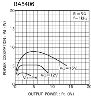
Fig.15 Power dissipation vs Output power(1)
