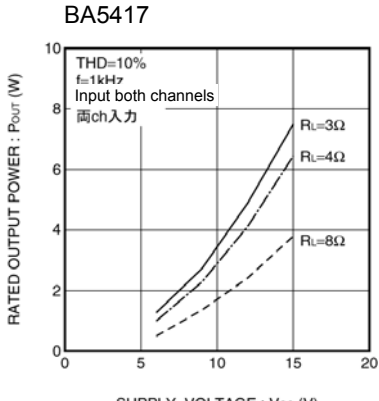
Fig.20 Rated output power vs Supply voltage
