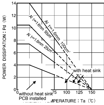
Fig.8 Thermal derating curve
