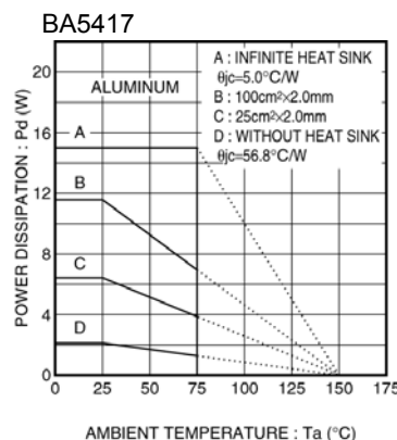
Fig.27 Thermal derating curve
