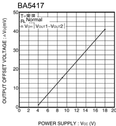
Fig.40 Output offset voltage vs. Supply Voltage
