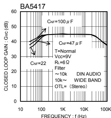
Fig.30 Closed loop gain vs. Frequency
