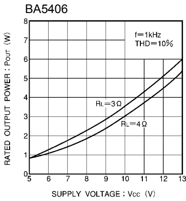
Fig.14 Output power vs power supply voltage
