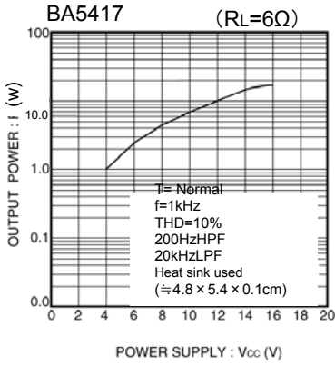
Fig.31 Rated output power vs. Supply Voltage
